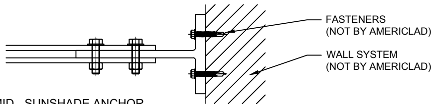
DETAIL @ MID - SUNSHADE ANCHOR
