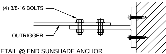
DETAIL @ END SUNSHADE ANCHOR
