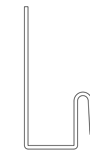
STARTER FLASHING PART# 8000-4
