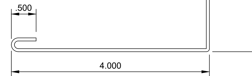
CORNER FLASHING PART# 8000-6 QTY: 10'-0" STOCK LENGTHS
