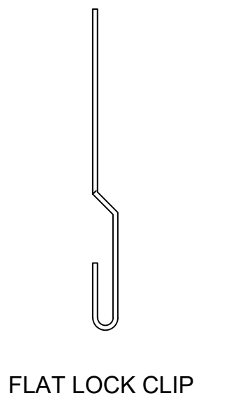
FLAT LOCK CLIP
