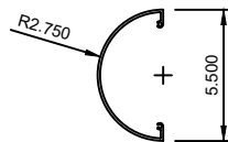
BULLNOSE FASCIA
